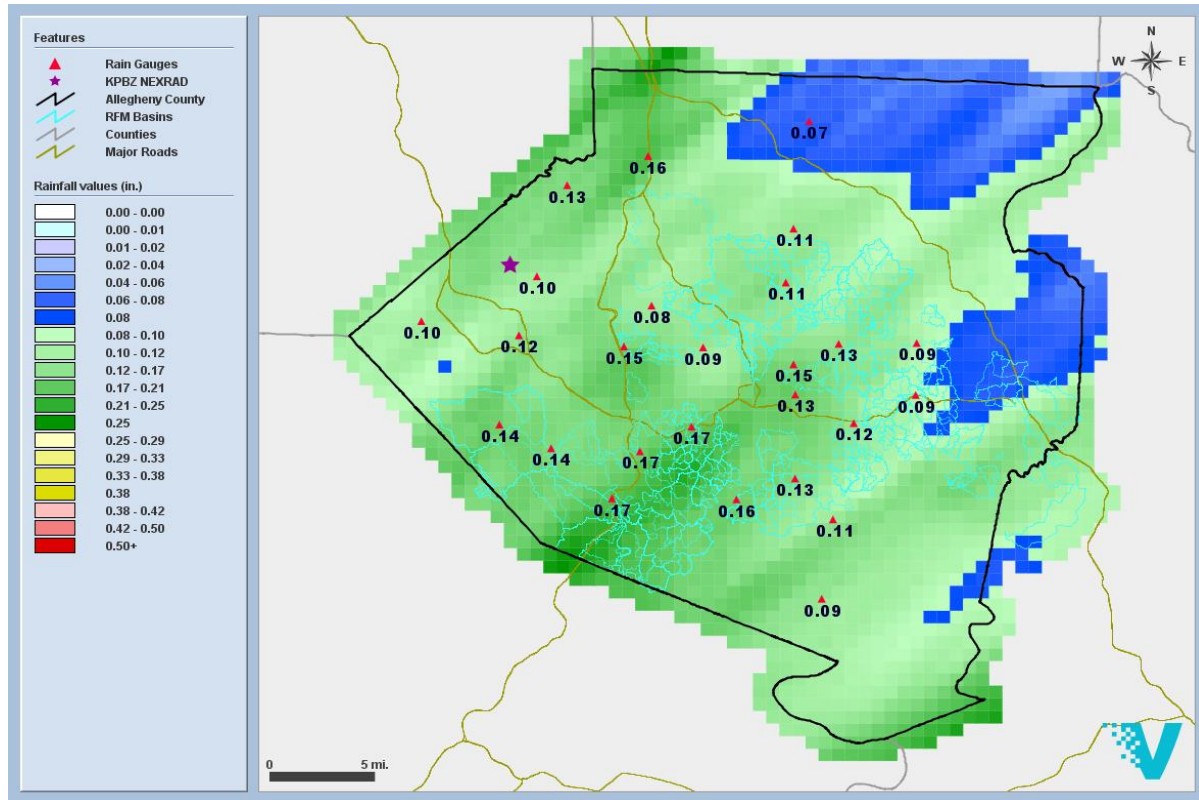
Figure 19. GARR Storm Total for Event 4
