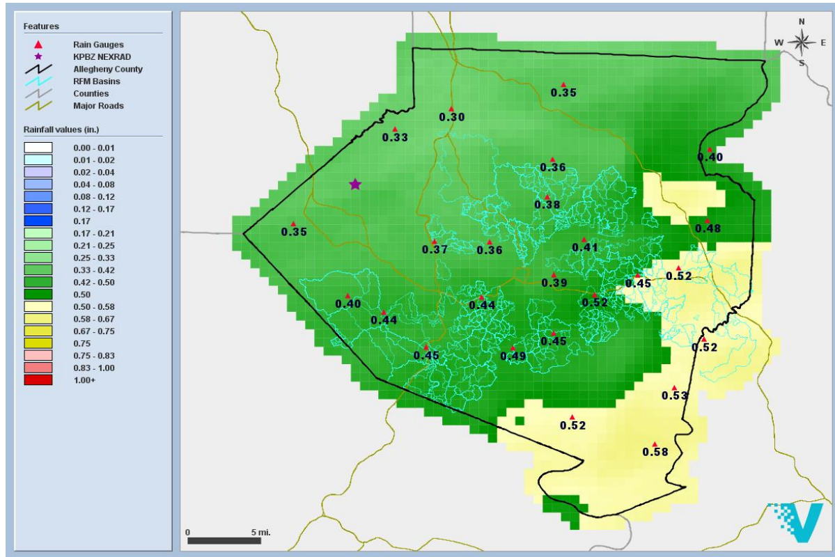
Figure 8. GARR Storm Total for Event 1
