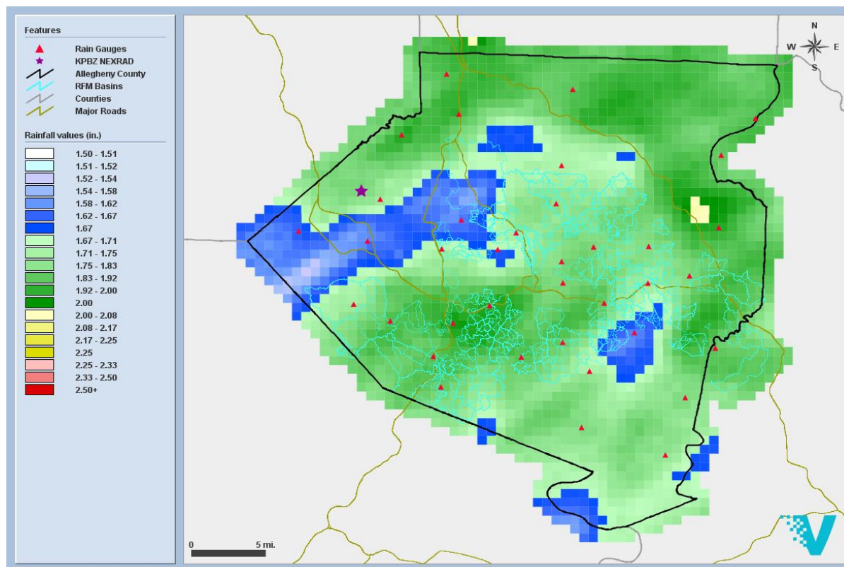
Figure 2. GARR Storm Total for November 2019
